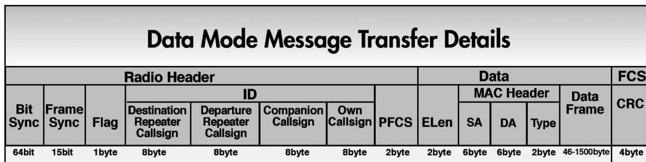
Fig 2—Proposed bit pattern in high-speed digital mode.
