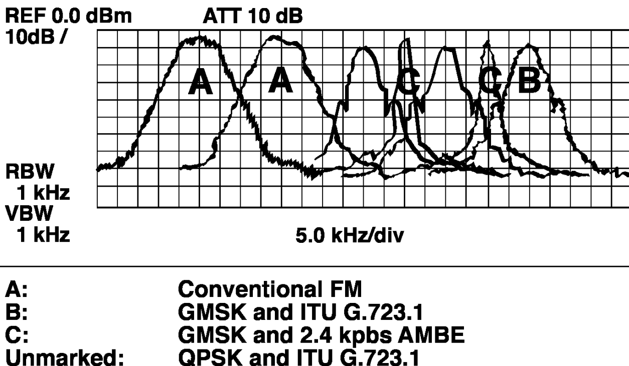
Fig 4—Occupied bandwidth of digital radio.
